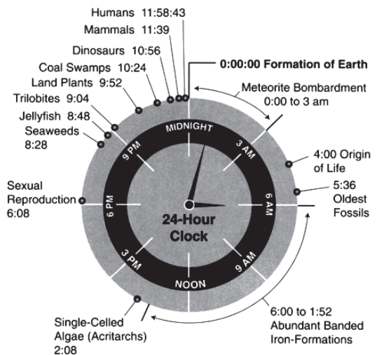
Fig 4.1. Formation of earth in an imaginative clock
