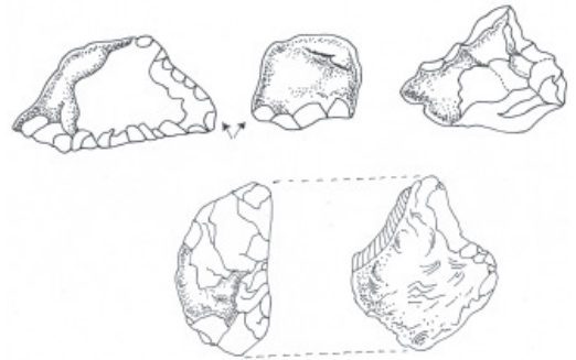
Fig. 4.6. Some eoliths
