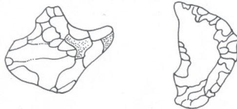
Fig 4.13. Clactonian tools
